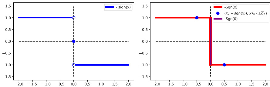
Fig. 1 The function -\text{sign}(x) and its (unperturbed) set-valued variant -\text{Sign}(x) (Color figure online)
