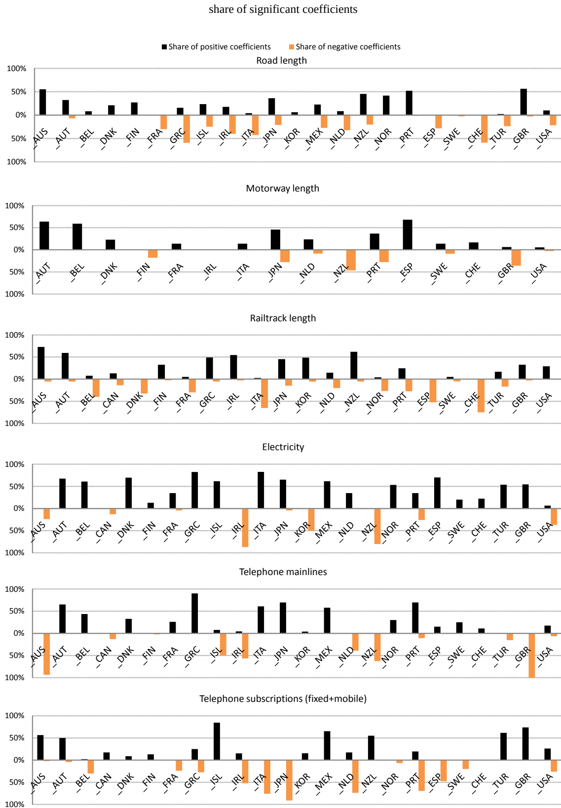
Figure 2. Robustness check for time-series growth regressions
