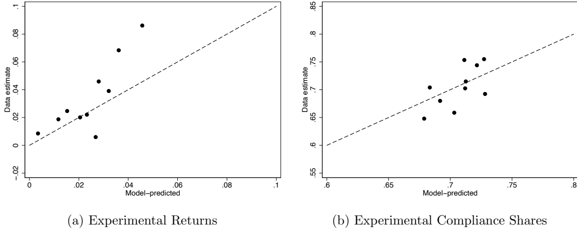
Figure A.6: Model-predicted Experimental Effects vs. Estimates from the Data
