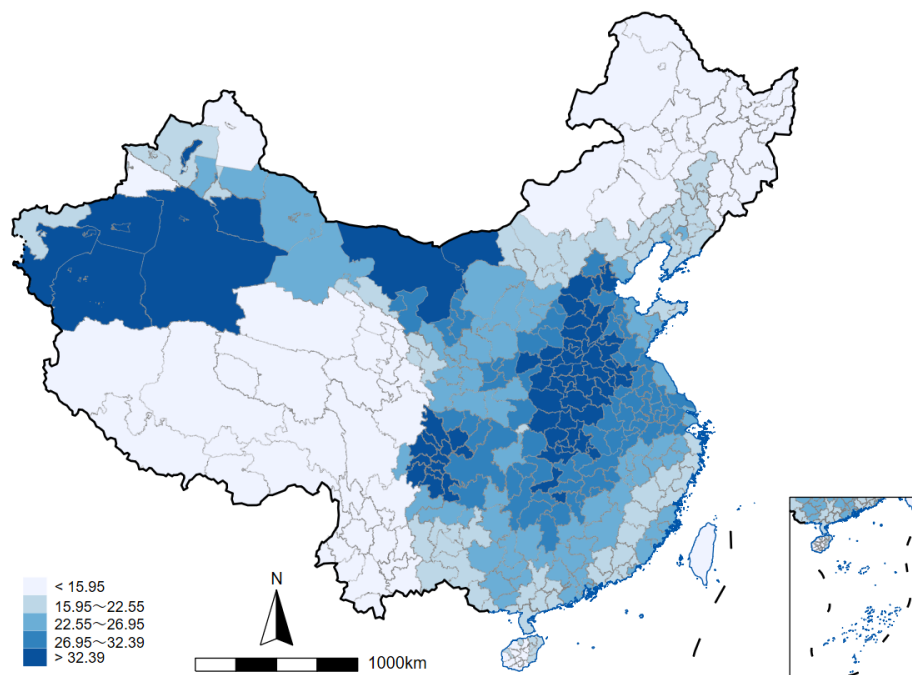
Figure A1: Spatial distribution of PM 2.5 ( \mu\text{g}/\text{m}^3 ) at city level during 1980-2000, China
