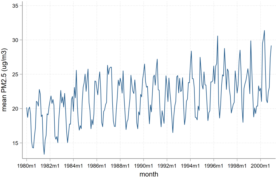
Figure A2: Monthly mean PM2.5 ( \mu\text{g}/\text{m}^3 ) during 1980-2000, China
