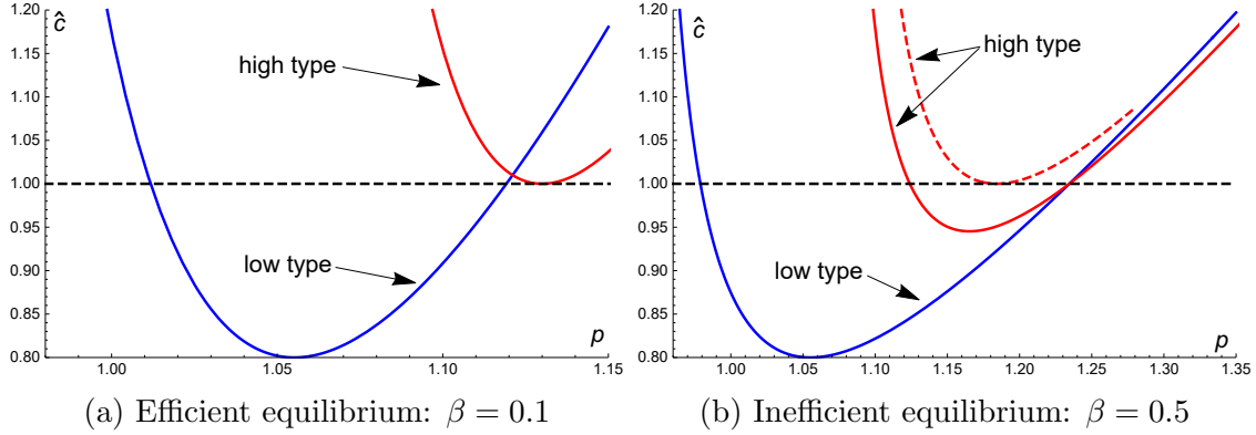
Figure 1: Illustration of the competitive search equilibrium with two types of sellers: m(\lambda) = 1 - e^{-\lambda} , k = 0.3 , c_1 = 0.8 , c_2 = 1 , v_1 = 1.5 and \nu(c) = v_1 + \beta(c - c_1) . To help compare figures (a) and (b), we set \hat{c} instead of \hat{v} as the y -axis where \hat{v} = \nu(\hat{c}) so that the positions of the black dashed lines in the two figures are the same.
