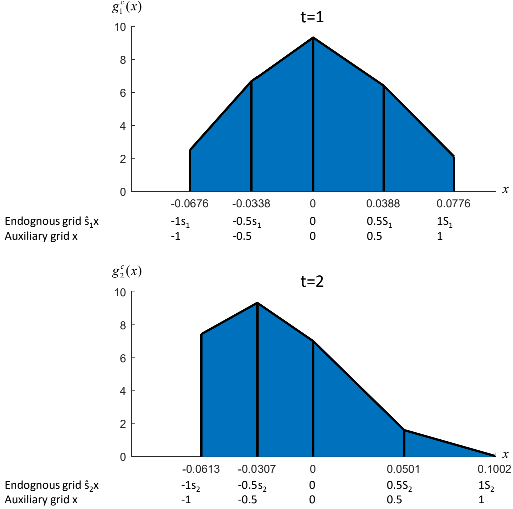
Figure 19: This figure schematically explains the linear interpolation with an endogenous grid. It shows the piece-wise linearly approximated distribution g_t^c(x) at two points in time, t = 1 and t = 2 . The thresholds of the (S, s) band are not symmetric around 0 and differ across time. The endogenous grid x has I grid points, which are automatically adjusted so that half of the grid points cover the negative part of the (s, S) band and half of them cover the positive part. In this illustrative example I = 5 (we use a larger I when solving the model). The adjustment is obtained by multiplying the auxiliary grid x = [-1, -0.5, 0, 0.5, 1] by \hat{s}_t(x) : x = x \hat{s}_t
