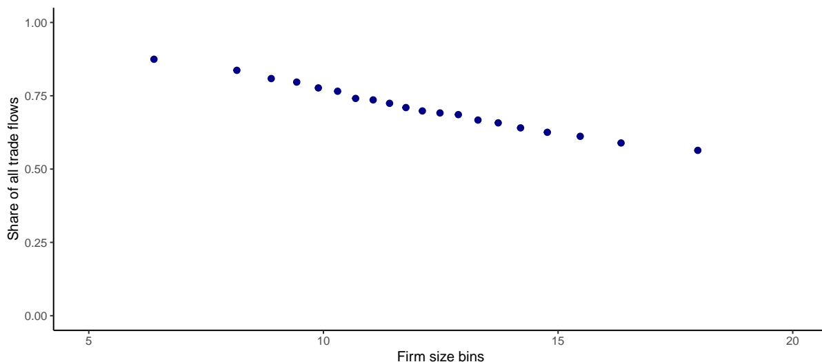
Figure 2: New trade flows
