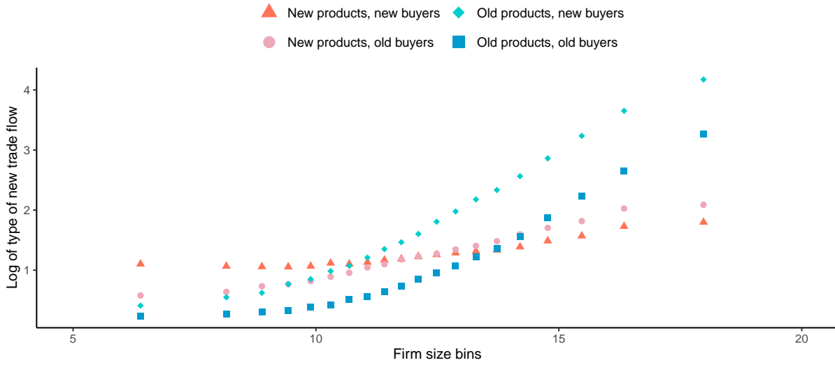
Figure A4: Composition of new trade flows: Absolute number
