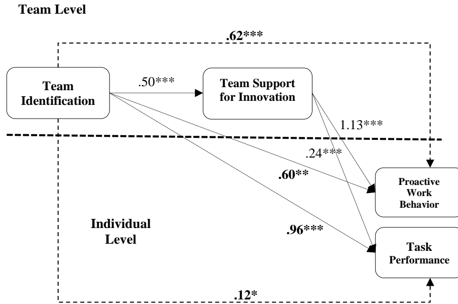
Figure 2: Hypothesized Results
