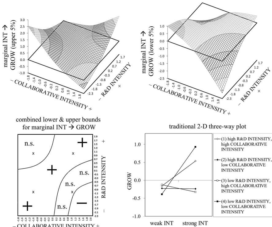
Fig. 2 3D and 2D plots of a three-way interaction
