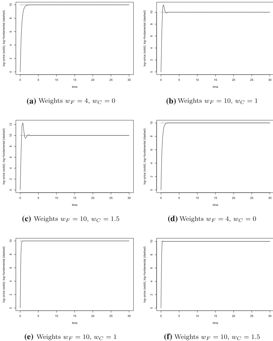
Fig. 8 Price dynamics for the implicit model with varying weights and step sizes, f = 10 and p(0) = 0 with step size h = 0.25 for (a–c) and step size h = 0.1 for (d–f)
