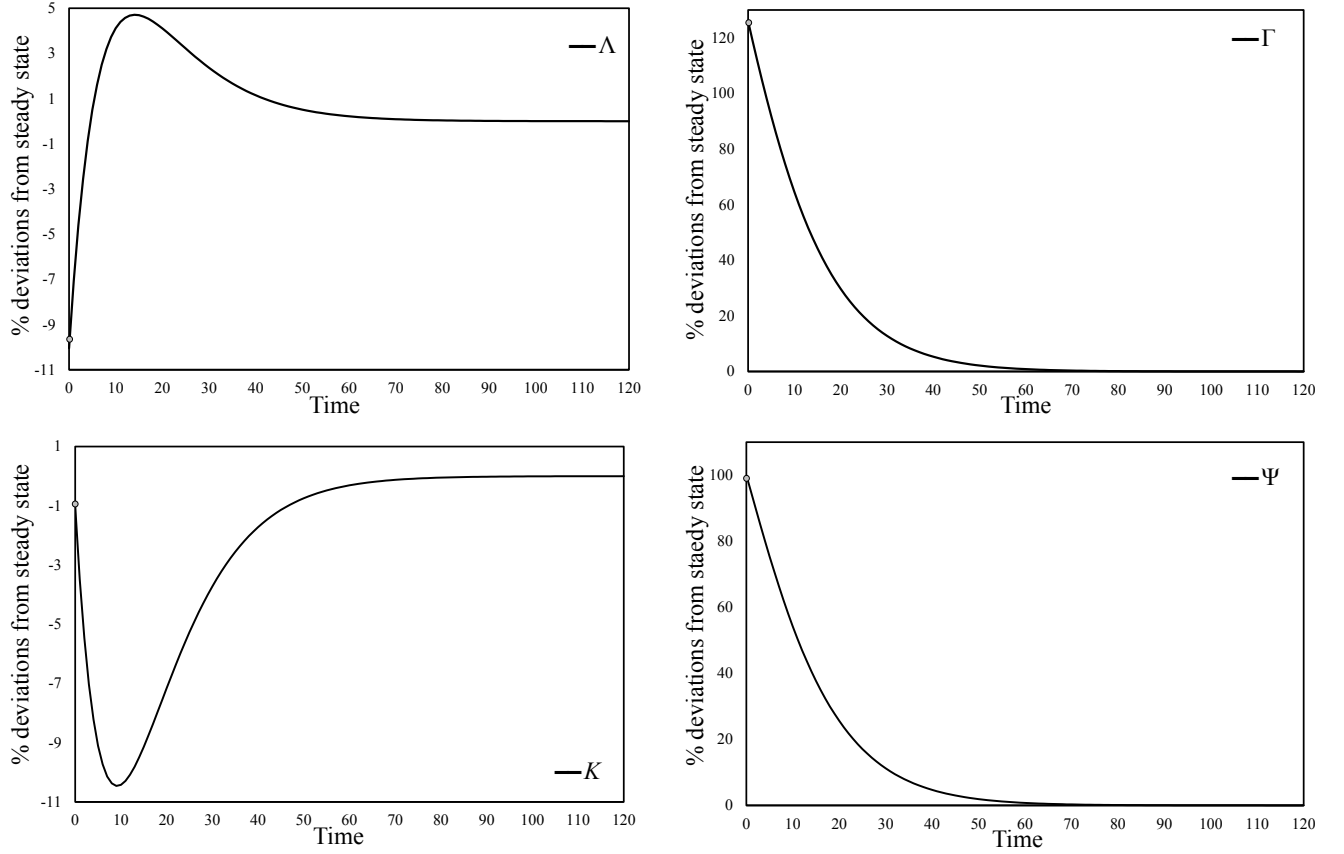
Figure 2: Saddle-path dynamics
