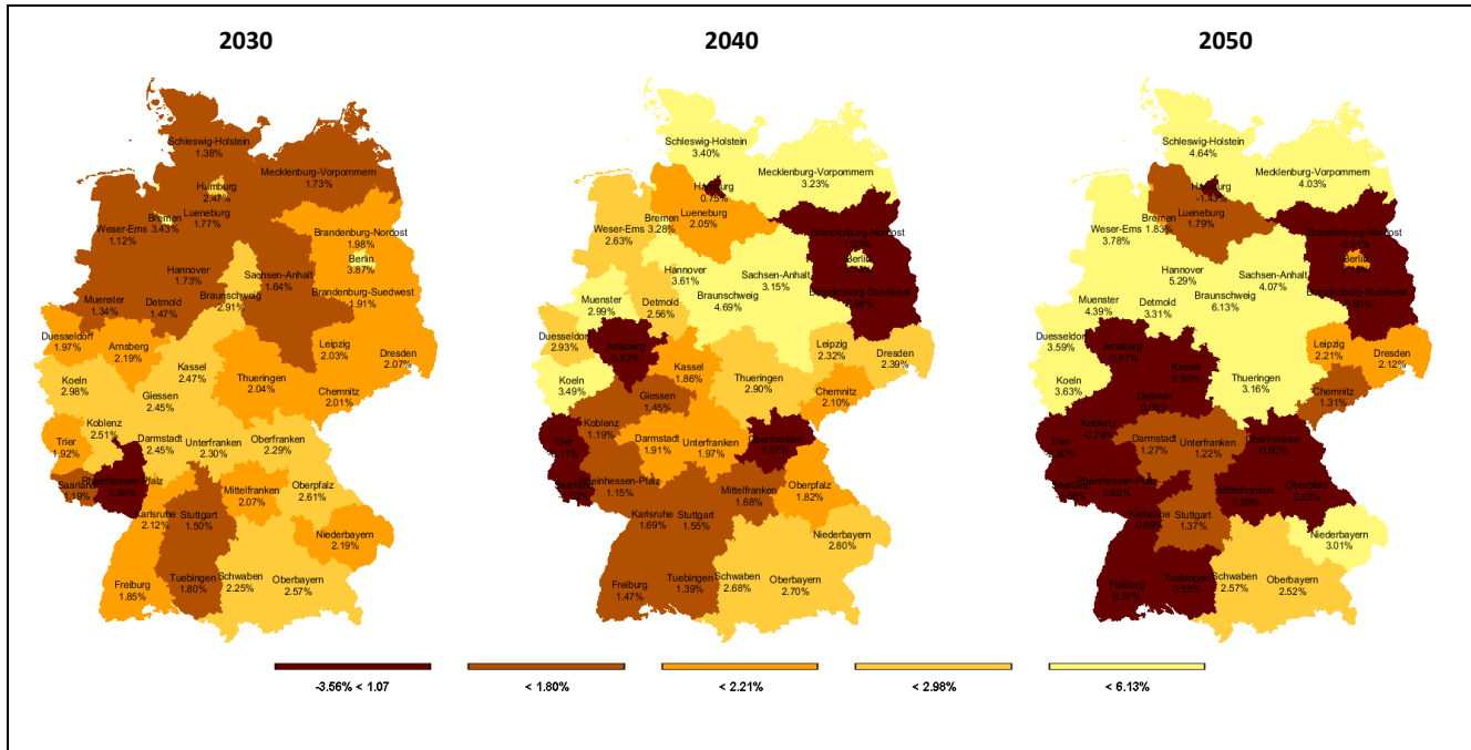
Figure 5. Percentage change in cropland compared to 2021 (baseline scenario)
