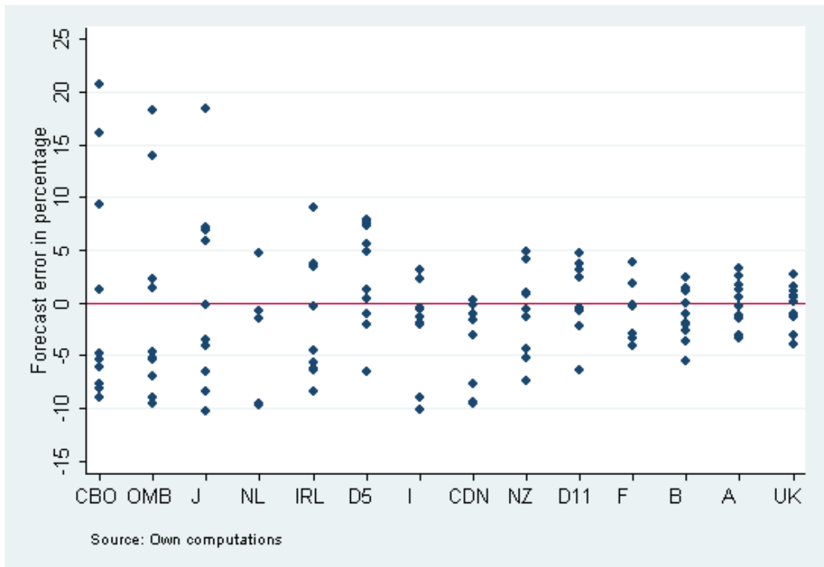
Figure 1: Forecast Errors
