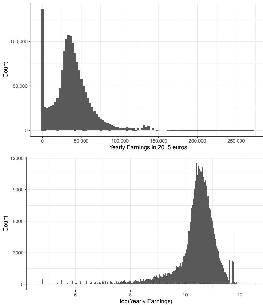
Figure A3: Earnings Distributions
