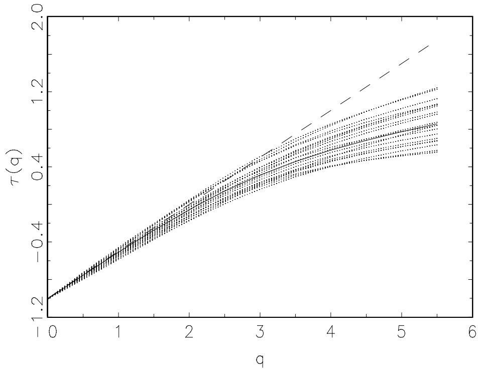
Scaling Function of Moments, NYCI
