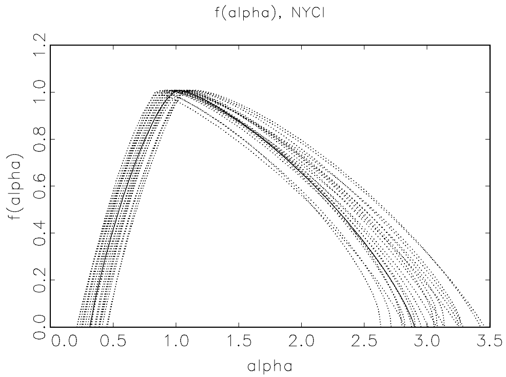
Fig. 2: f(\alpha) spectrum for New York Stock Exchange Composite Index returns (solid line) and twenty reshuffled series (dotted lines).
