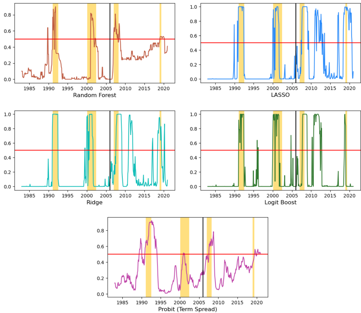
Figure 4: Recession Probability Plots
