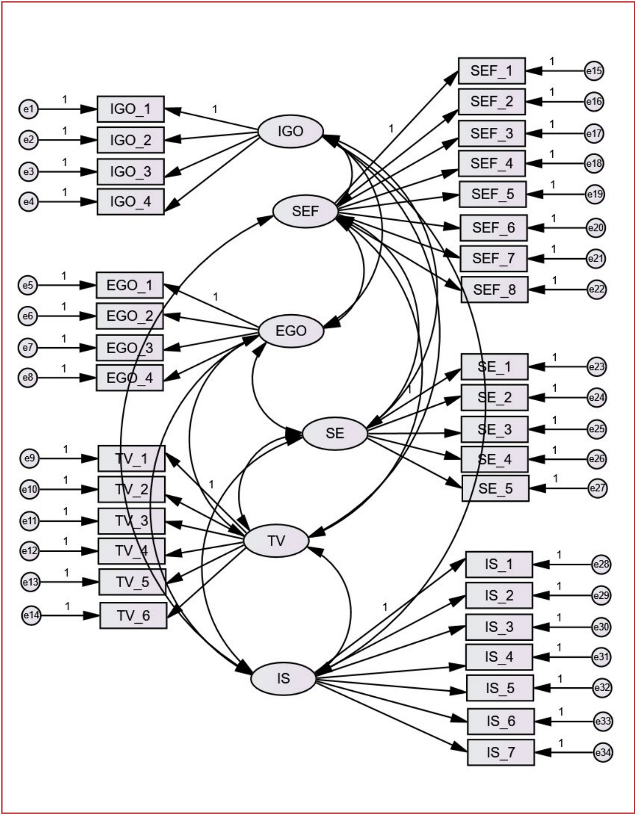
Figure 1 Visual overview of the model used in the factor analyses
