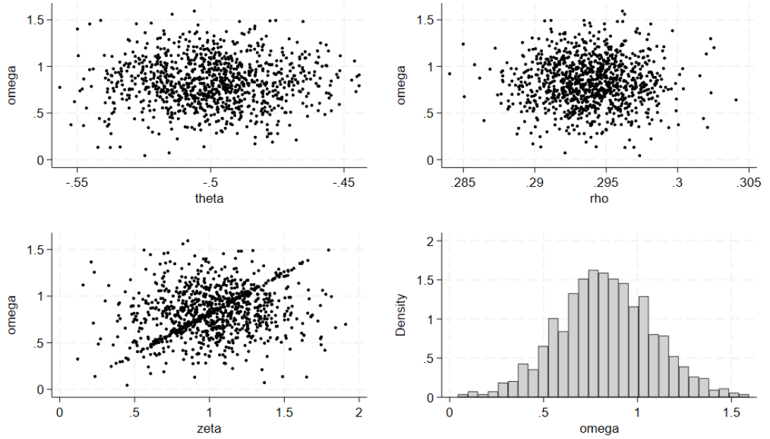
The figure presents Monte Carlo simulation results over 1000 estimations of Eq (A25) with different values of parameters rho, zeta and omega.
