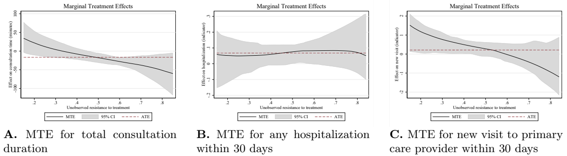
Figure A3. Marginal Treatment Effects (MTEs)
