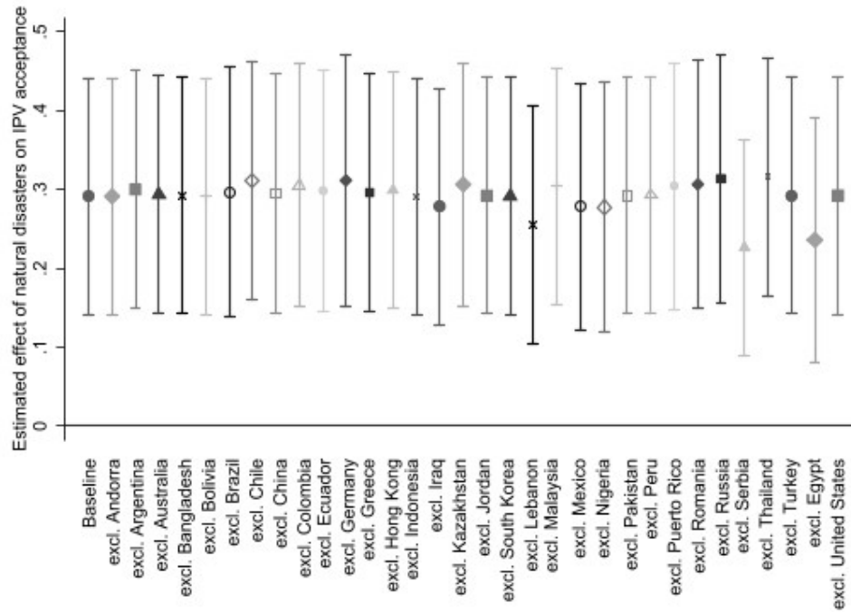
Figure 5. Results with leaving one country out of the sample at a time
