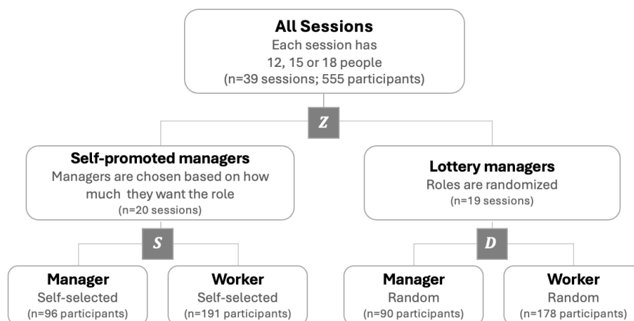
Figure 2: Randomization scheme
