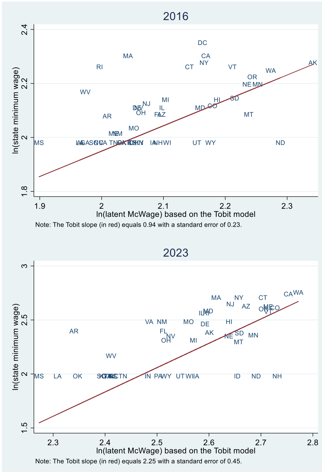
Fig. 3: State Minimum Wage Levels and Latent McWages
