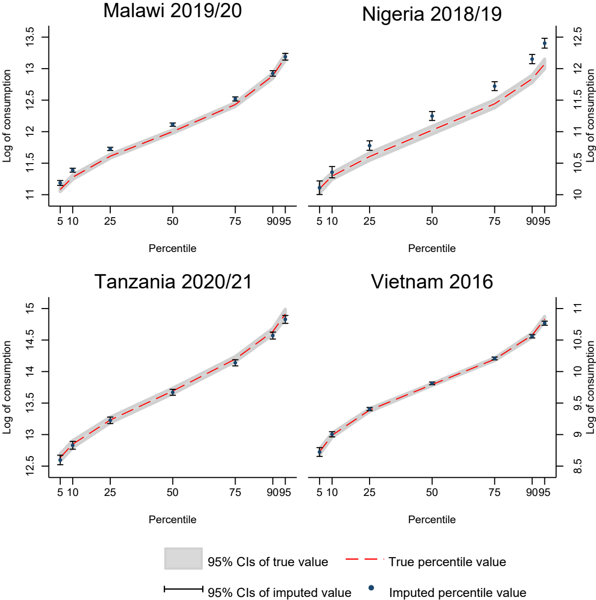
Figure A.2. Predicted consumption distribution, Model 9
