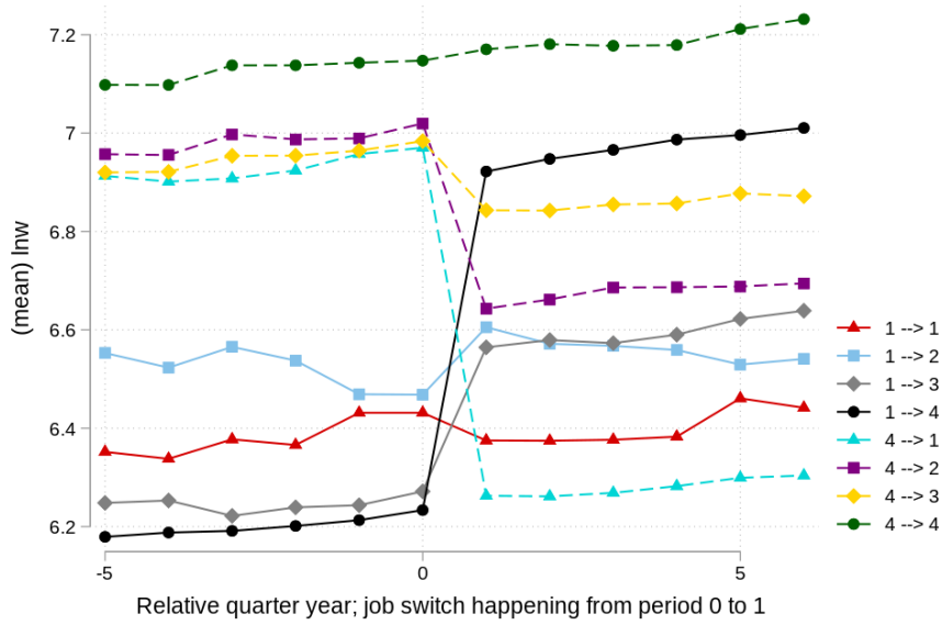
Figure B2: Event study of Card et al. (2013)
