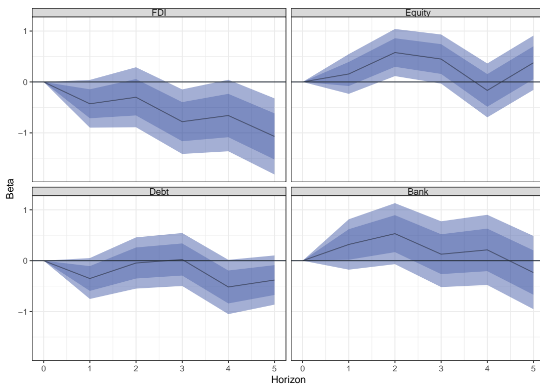
Figure A7: Local Projections with Balanced Sample
