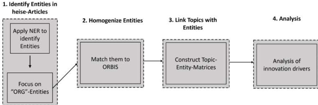
Figure 4: Visualization of the Entity Analysis Pipeline
