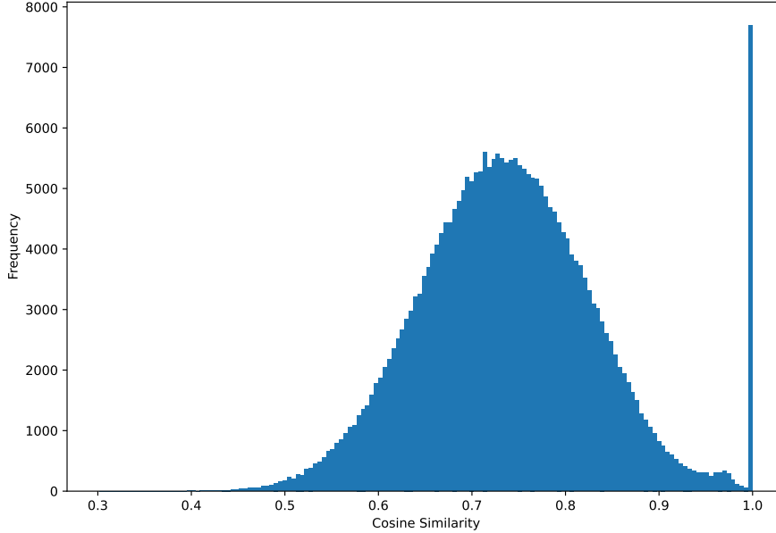
Figure 6: Histogram of pairwise cosine similarities for the highest cosine similarity for each Heise entity
