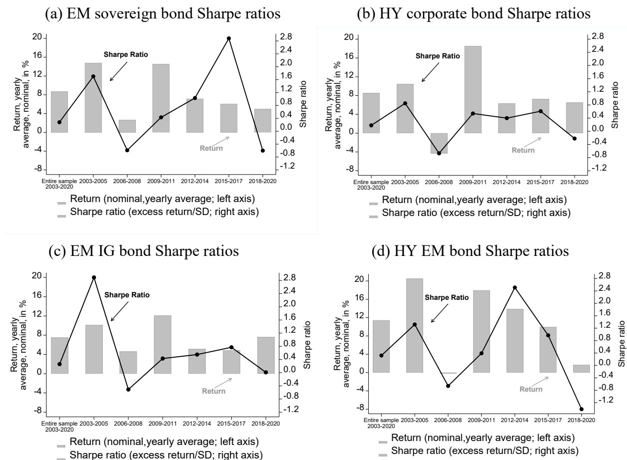
Figure 6. Sharpe ratios
