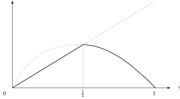
Figure 6: Profile of the minimized loss L^*
