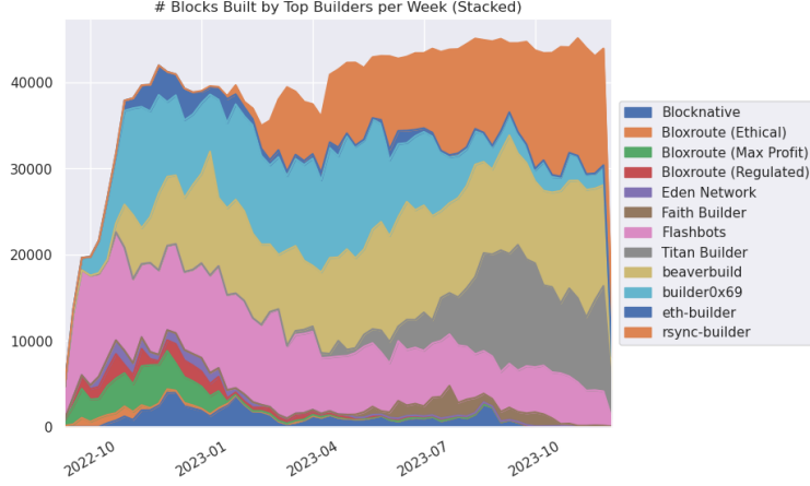
Figure 8: Block building concentration
