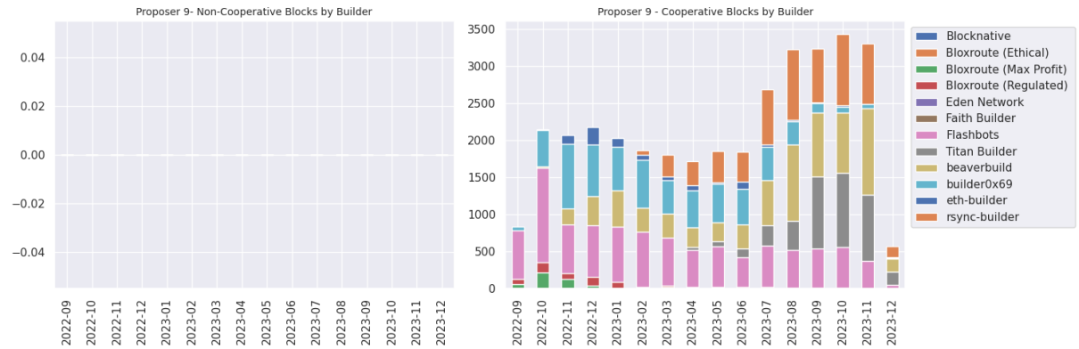
Figure 13: Non-cooperative and cooperative blocks by other proposer
