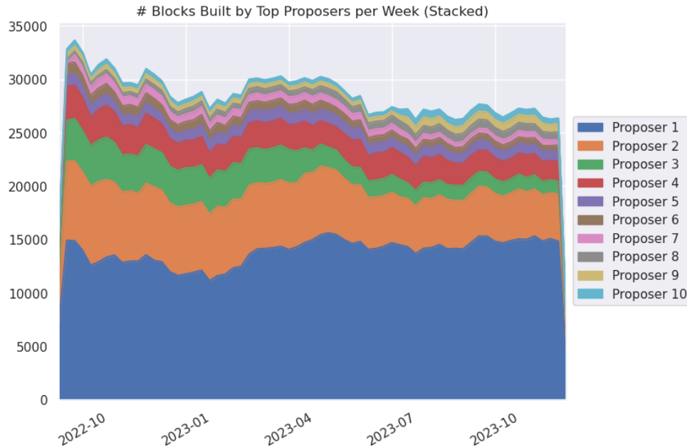
Figure 10: Block proposer concentration
