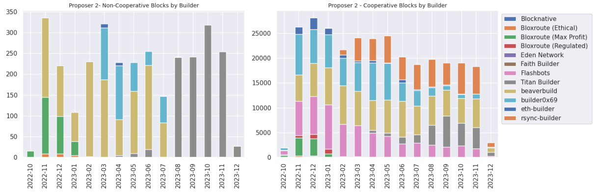
Figure 12: Non-cooperative and cooperative blocks by Proposer 2
