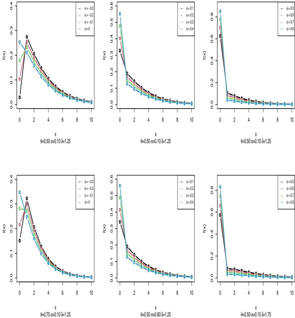
Figure 1: The pmf of the ZMPMQL distribution at different parameter values of \phi , \theta , \alpha , and \delta
