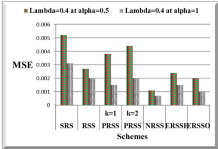
Figure 7. MSE of \hat{\lambda} for all schemes at m = 100
