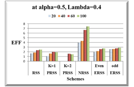
Figure 11. Efficiency of the MLEs for all schemes at all sample sizes
