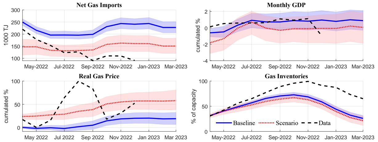
Figure A.9: Conditional forecasts for a natural gas embargo against Russia starting in April 2022
