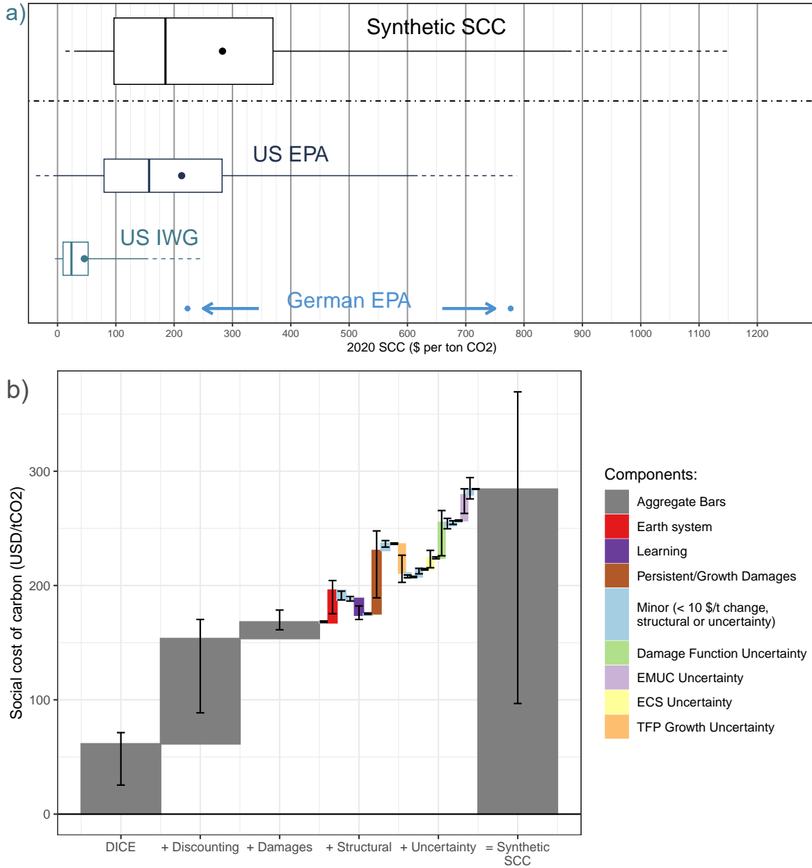
Figure 5: Synthetic 2020 SCC Distribution and Decomposition. a) Synthetic SCC distribution generated from the random forest model forced by input distributions over model structure and discounting shown in 3c and d. 2020 SCC distributions from two US government SCC assessments, a 2023 EPA analysis [54] and the 2021 update from the Interagency Working Group [51]. Boxplots show the median (line), inter-quartile range (box), 5-95% range (solid line) and 2.5-97.5% range (dashed lines). Dots show the mean after trimming the upper and lower 0.1% of each distribution. Dots show the two SCCs provided by the German EPA [55] under two pure rates of time preference (0% and 1%). b) Decomposition of the difference in the synthetic SCC distribution and the random forest predictions given inputs (over model structure, discounting, damages, and treatment of uncertainty) corresponding to the DICE model [52]. Because of interactions, the decomposition depends on the order in which elements are added. Figure shows values averaging over interaction effects using 30 randomly selected different orderings. Error bars show the interquartile range.
