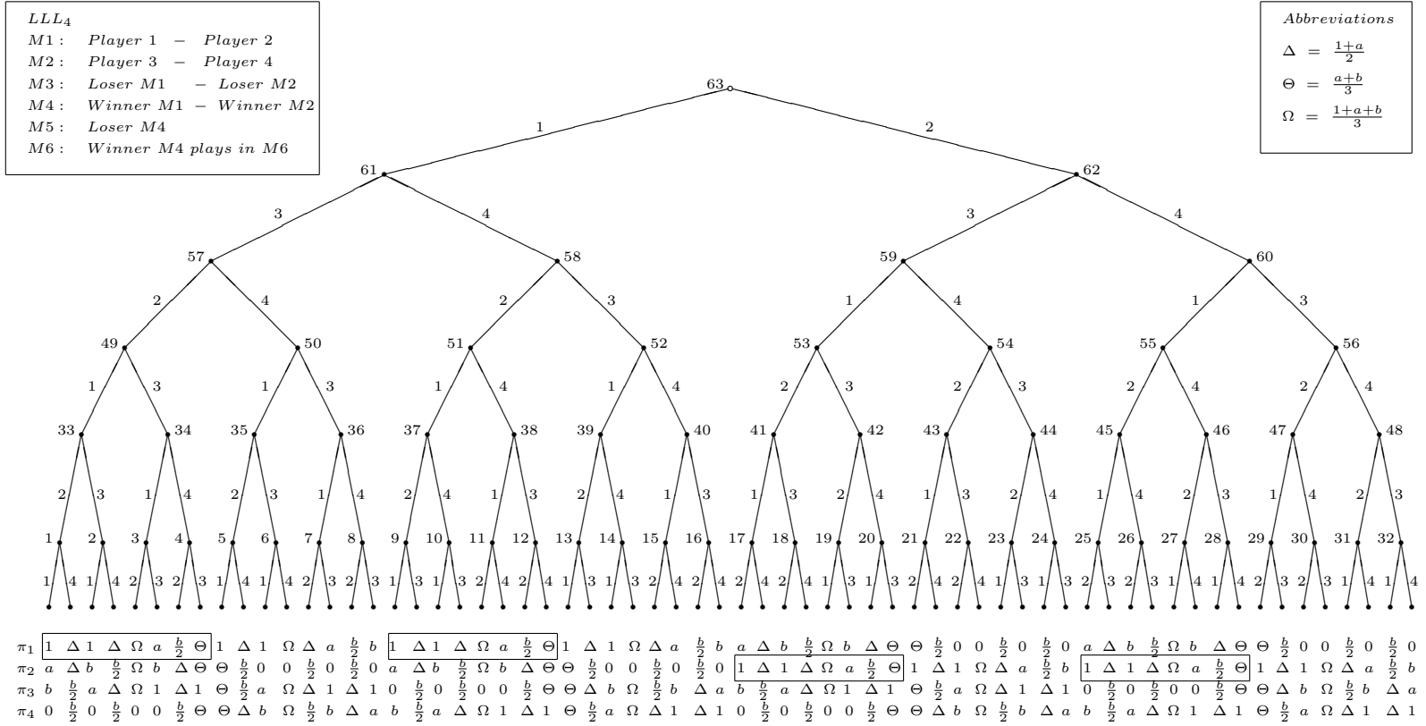
Figure 11: Game tree for LLL_4 : in boxes find payoff sequence A
