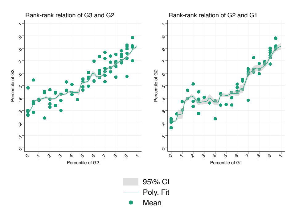
Figure A.3: Mean Child Percentile against Parent Percentile for six countries: Non parametric fit
