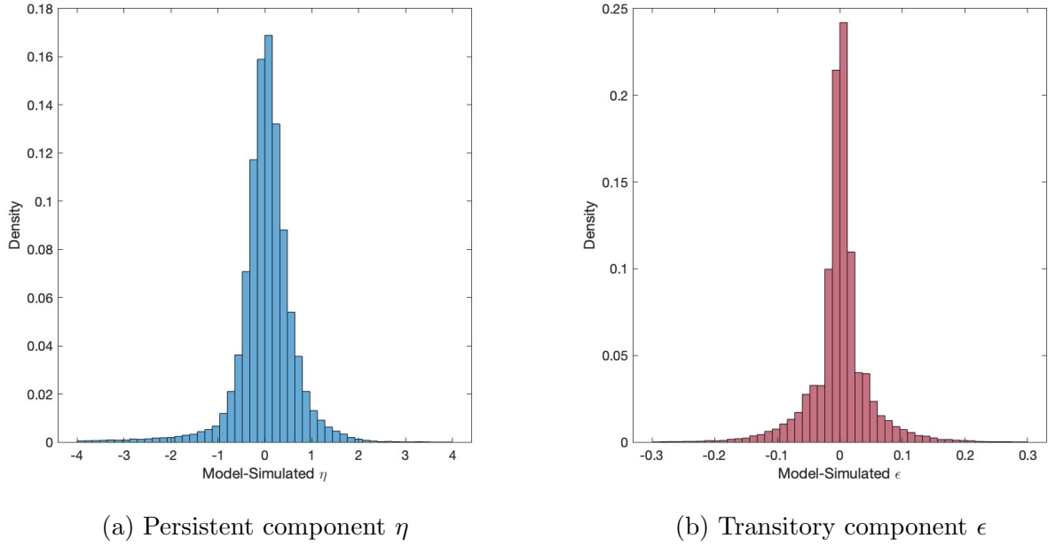
Figure A.13: Distribution of productivity components in the model
