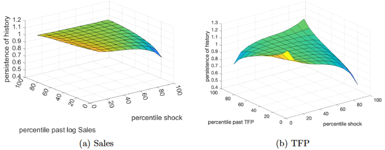
Figure A.7: Quantile autoregressions: all industries
