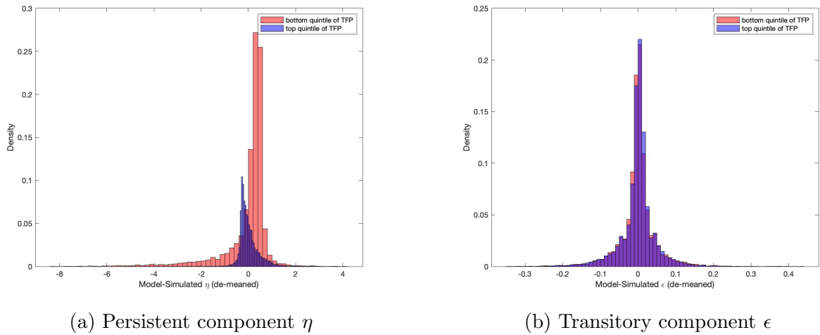
Figure A.14: Distribution of productivity components in the model by top and bottom quantiles of TFP
