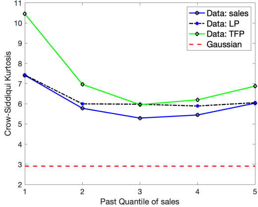
(c) Crow-Siddiqui Kurtosis
