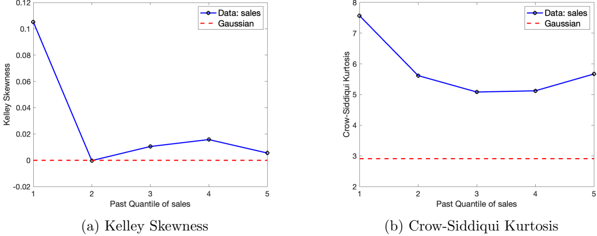
Figure 2: Skewness and kurtosis of one-year log sales changes
