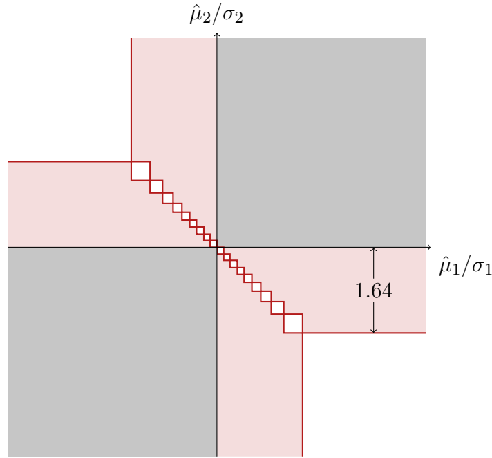
FIGURE 3.—A test with uniformly exact size control (i.e., constant rejection probability of 5%) on the boundary of H_0 . Here, H_0 is gray (positive and negative quadrant) and the nonrejection region beyond H_0 is red (irregularly shaped object in second and fourth quadrants).
