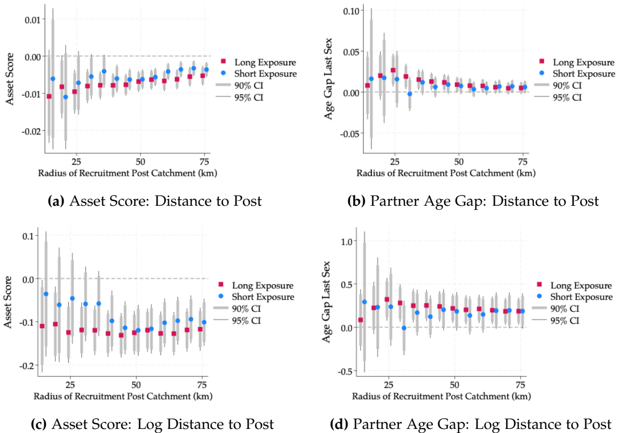
Figure J1: Varying Catchment Radius and Distance Measure [33]
