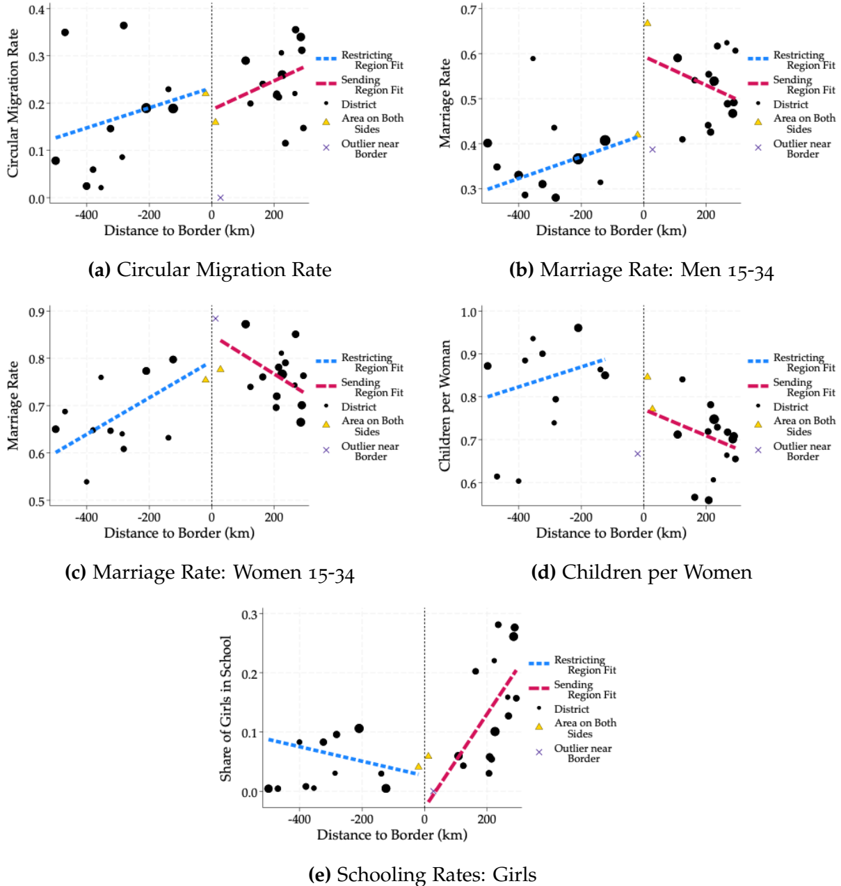
Figure H3: 1960 RD Plots [30]
