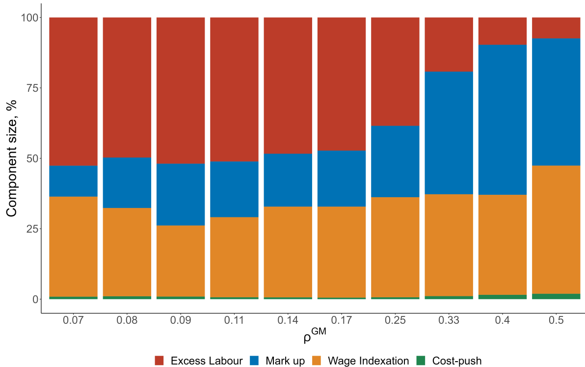
Figure 8: Absolute value of the Monte Carlo averages of the components of firm-level price growth as a function of the degree of imperfection in the market selection process in the goods market. Higher values of \rho^{GM} imply a more imperfect market selection process.
