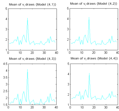
Figure 5: Computation of v_i draws of \Omega
