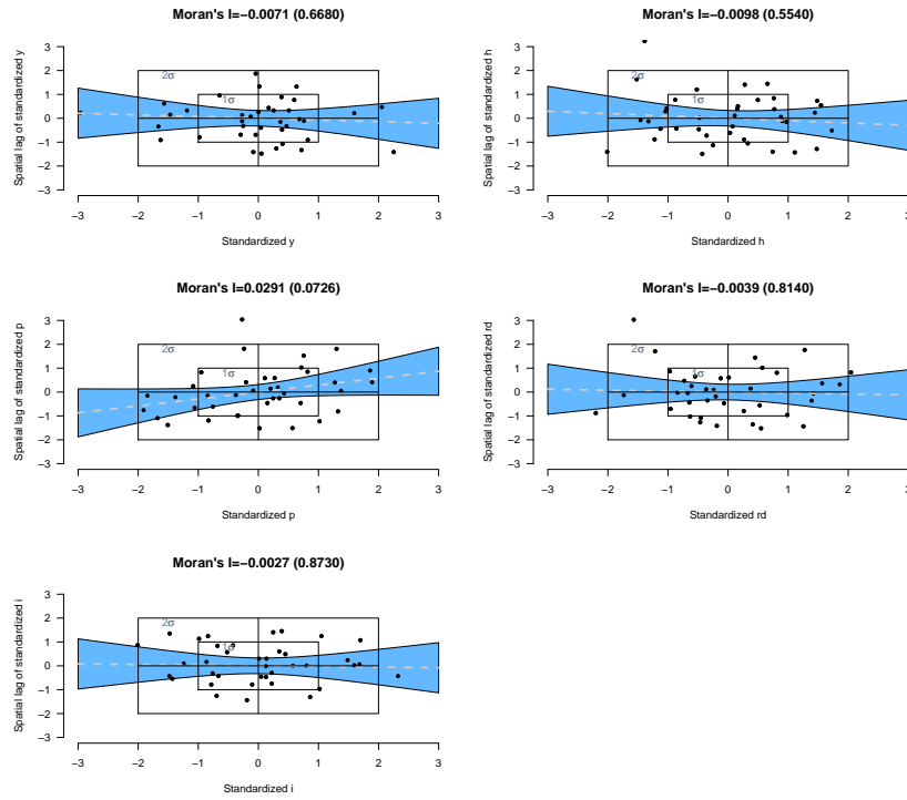
Figure 2: Computation of Moran's \mathcal{I} with corresponding p -values for dependent and independent variable for r = 2
