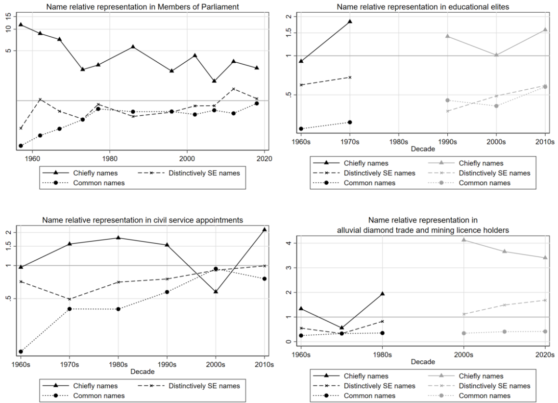
Figure B.3: Relative Representation of Rare Chiefly Names Compared with Relative Representation of Distinctively South-Eastern Names
