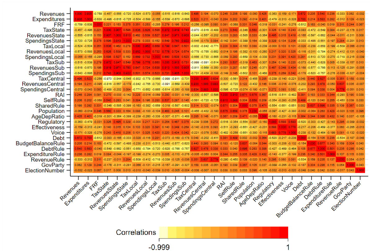
Figure 1: Heat map of Correlation Coefficients
