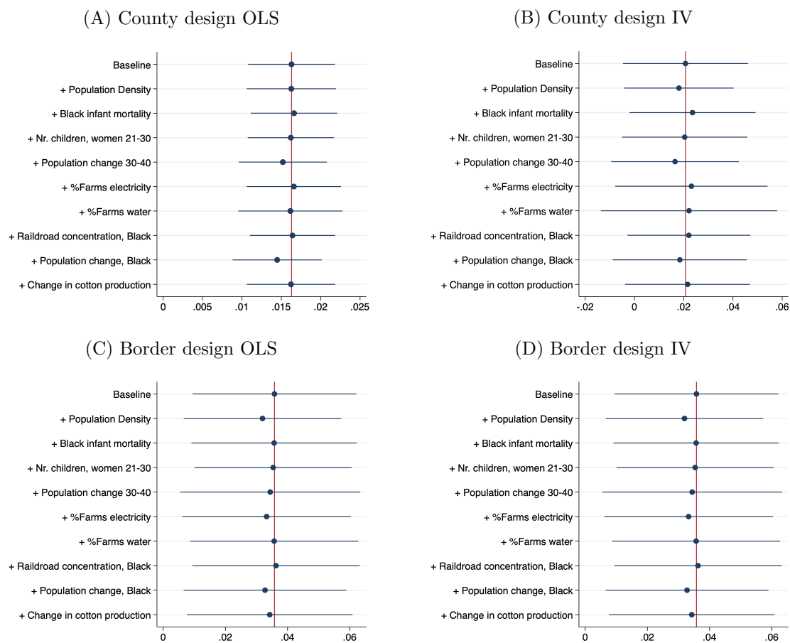
Figure 8: Sensitivity of Regression Estimates to the Inclusion of Additional Covariates
