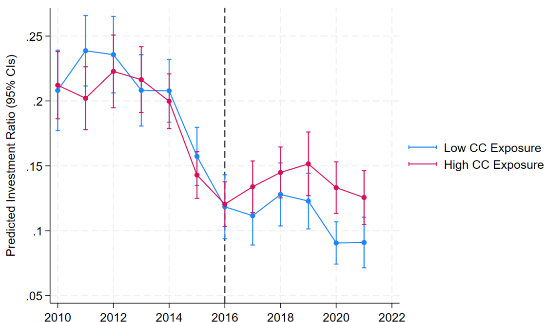
Figure 5: Parallel Trends
