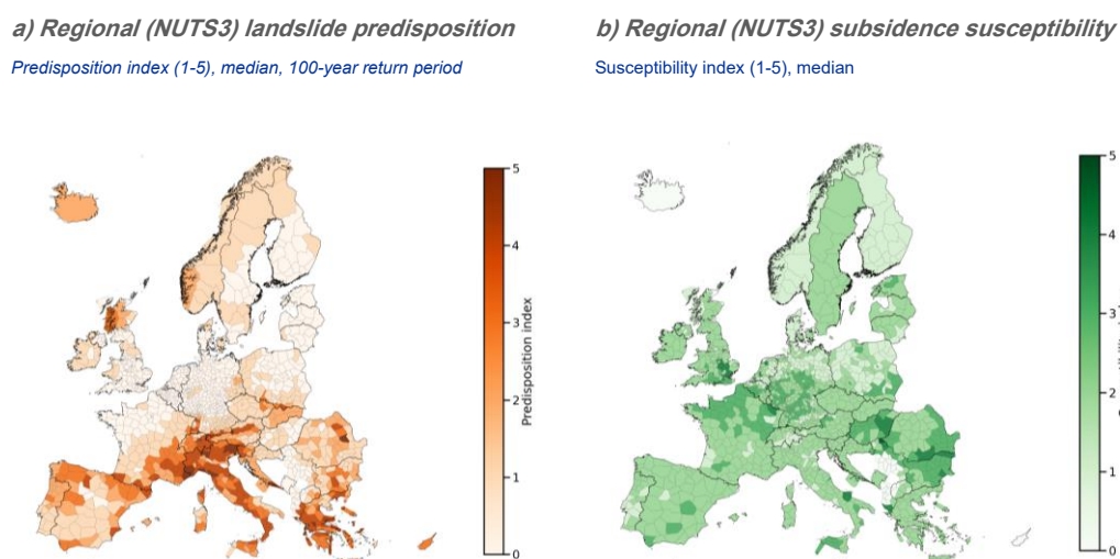
Figure 22 Landslides and subsidence risk scores
