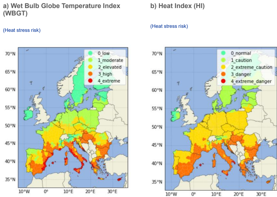
Figure 30 Projected heat stress risk derived from WBGT and HI for July and August 2100 and SSP-5 RCP-8.5 scenario
