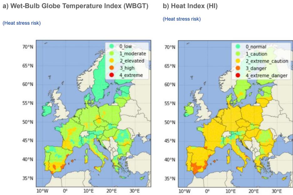
Figure 29 Historical heat stress risk derived from WBGT and HI recorded during July and August 2003
