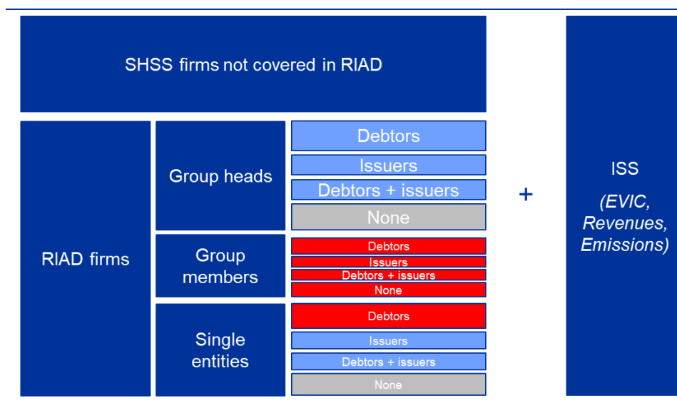
Figure 45 Construction of the group frame for group-level imputations
