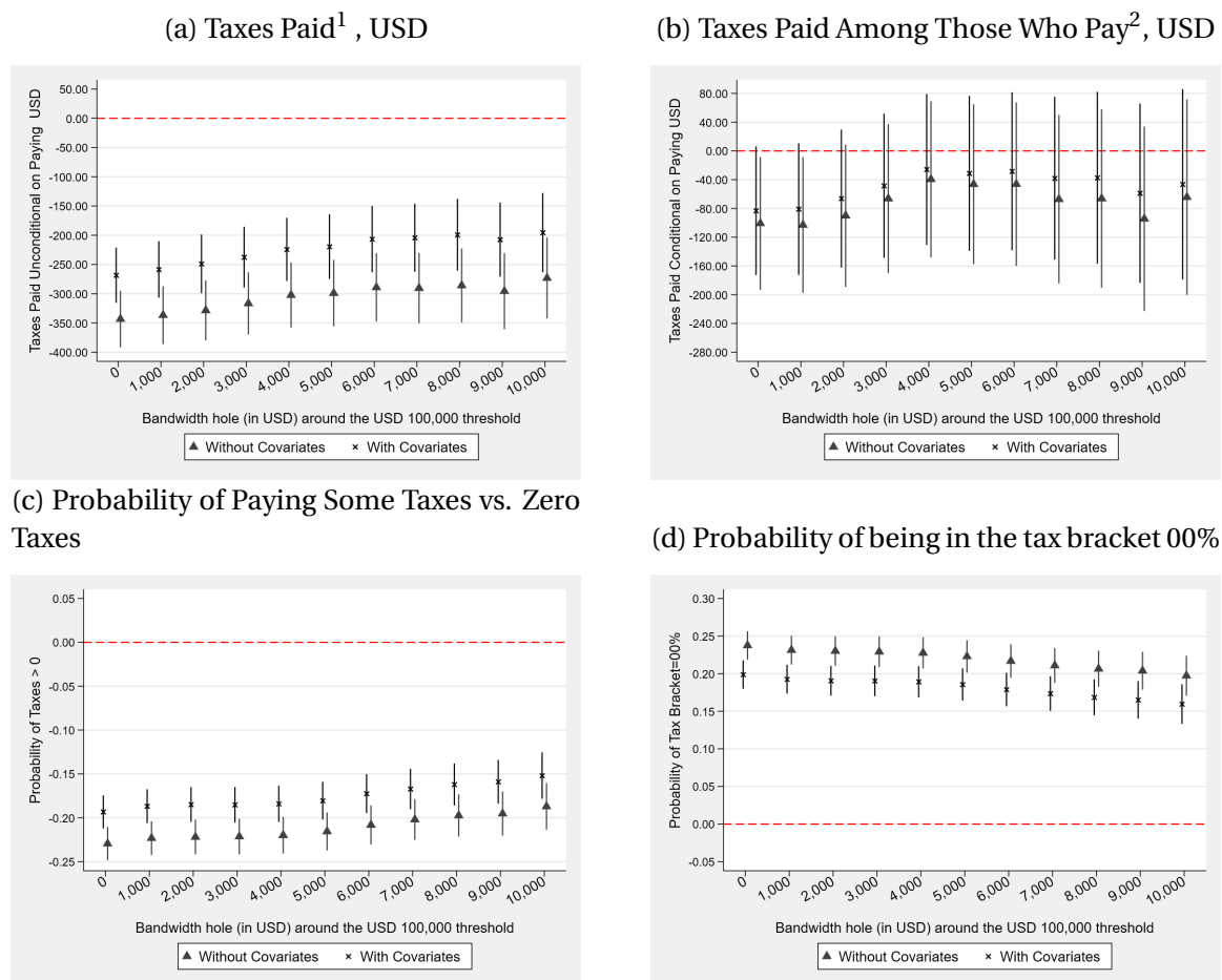
Figure 6: Donut estimator - First Approach
