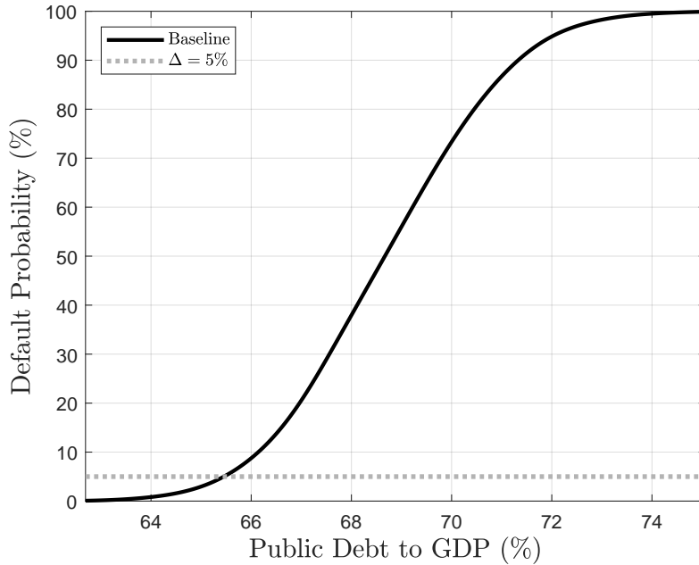
Figure 3: Baseline Fiscal Limit Distribution
