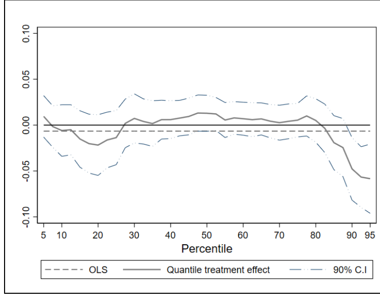
Figure 5. Placebo test: Pre-treatment quantile treatment effects
