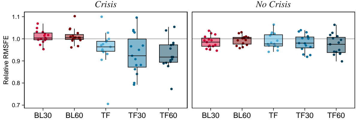
Figure 6: Boxplots of the relative RMSFE across Specifications against the Baseline Specification
