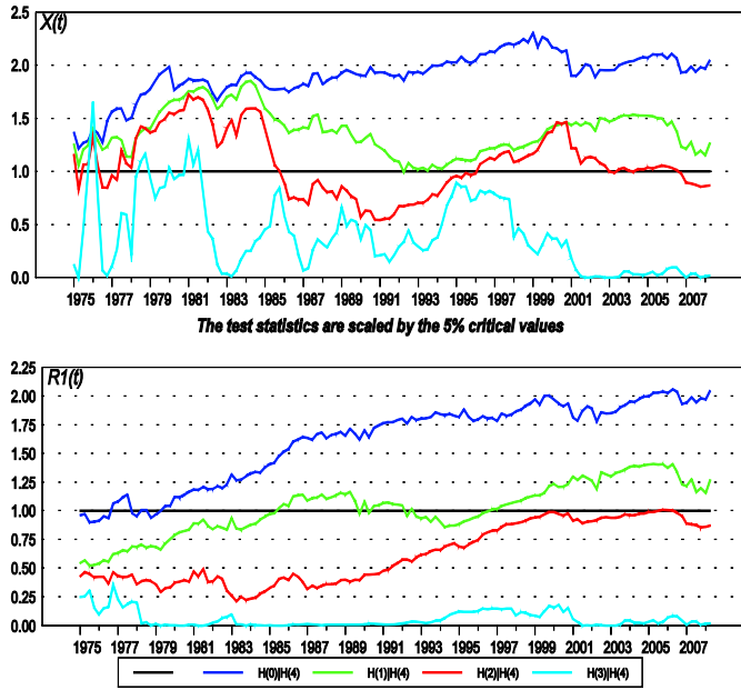
Figure 3: Recursive calculated trace test statistics based on the full and the concentrated model (Base sample 1970:03 to 1975:1) for CRBRI
